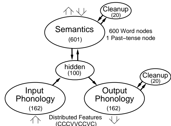
Figure 5. The architecture of the network used by Joanisse and Seidenberg (1998) to model inflectional morphology. The number of units in each layer is indicated in parentheses. The small black arrows indicate full connectivity from one group of units to another. The large open arrows identify groups of units that receive input (incoming arrow) or generate output (outgoing arrow). Input and Output Phonology are represented in terms of distributed features, whereas Semantics encodes each concept by the activation of a single node (plus a past-tense node when appropriate). (Adapted from Joanisse & Seidenberg, 1998)
