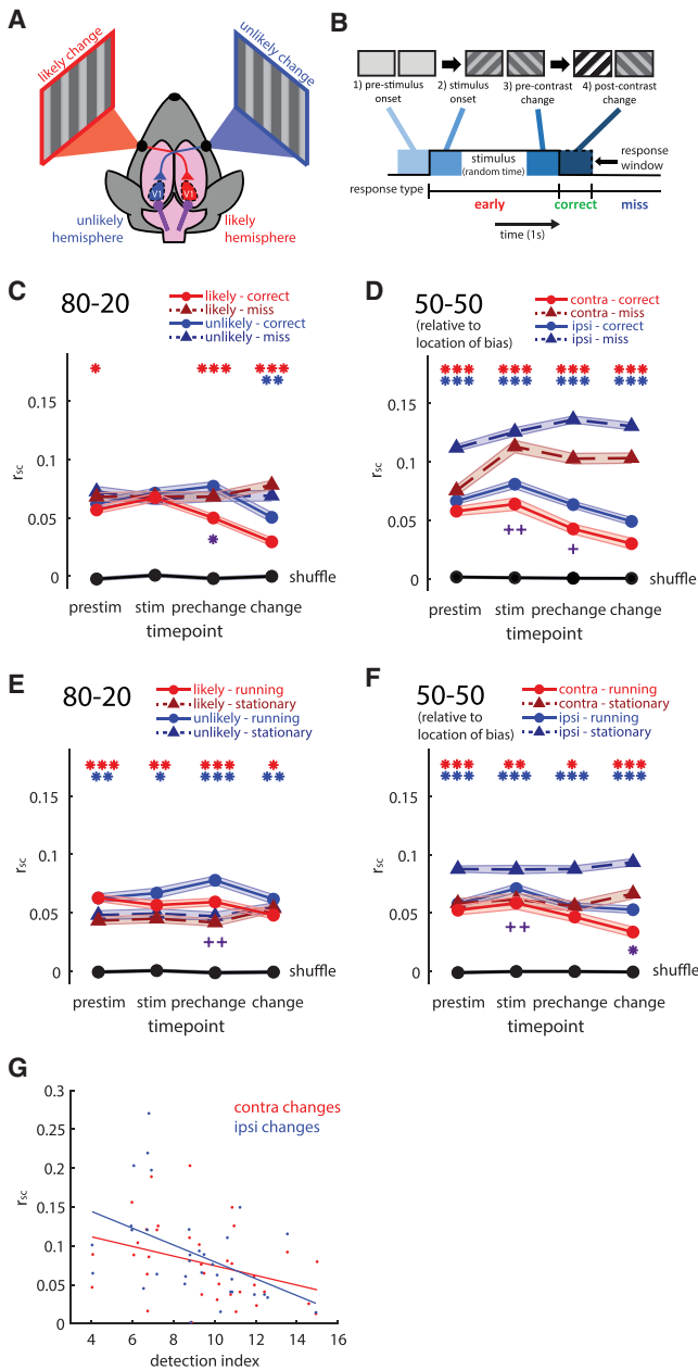
Figure 2. Local and Global Modulation of Correlated Variability
