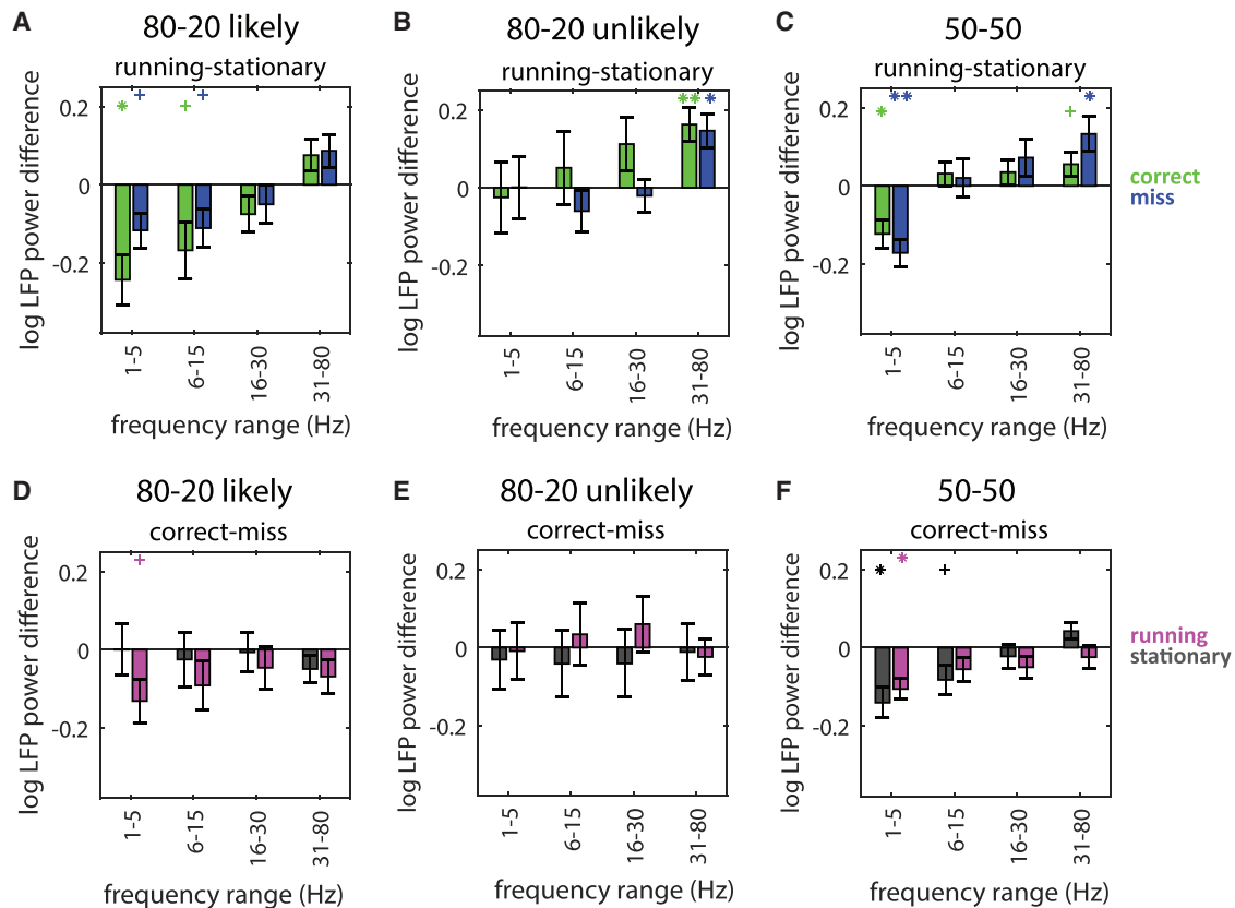
Figure 6. LFP Power Changes Consistently with Locomotion
