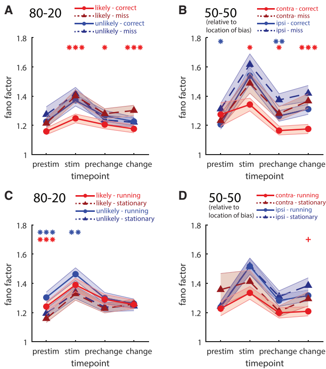
Figure 5. Local and Global Decreases in Individual Variability
