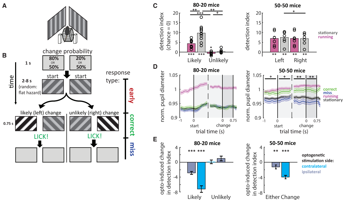
Figure 1. Spatial Selection Task and Behavioral Performance
