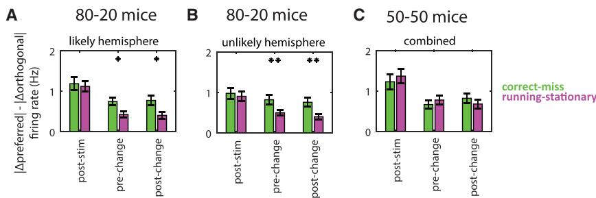
(C) In 50-50 mice, effects of selection (correct versus miss trials) and locomotion (running versus stationary) were not significantly different ( N = 177 significantly tuned neurons). * p < 0.05 , ** p < 0.01 , Wilcoxon signed-rank test between (correct-miss) and (running-stationary).
