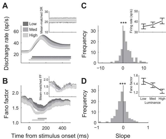
Fig. 4. Effect of luminance on discharge rate and Fano factor. A : mean discharge rate ( \pm SE) divided by target luminance (low, 0.01–0.6 \text{cd/m}^2 ; medium, 0.20–1.00 \text{cd/m}^2 ; high, 1.70–5.00 \text{cd/m}^2 ). Gray circles indicate significant differences from baseline (Wilcoxon rank-sum test, P < 0.01 ). Inset shows mean-matched discharge rate for each luminance group (see METHODS; Churchland et al. 2010). The mean-matched discharge rate is invariant across time and luminance. DR, discharge rate. B : variations in Fano factor with luminance. Conventions are as described in A . Fano factor decreases significantly with luminance even when controlling for changes in mean discharge rate. FF, Fano factor. C : distribution of slopes of mean discharge rate as a function of luminance group in the poststimulus epoch (spikes/s per \text{cd/m}^2 ). Inset shows mean discharge rate ( \pm SE) by luminance group. ***P < 0.001 , significant difference of mean value from 0 (Wilcoxon signed-rank test). D : same as C but for Fano factor (Fano factor per \text{cd/m}^2 ). Note that discharge rate and Fano factor were computed using 150-ms time bins; therefore, the visual latency may appear earlier due to temporal smearing. All latency estimates reported in text used smaller 50-ms time bins.
