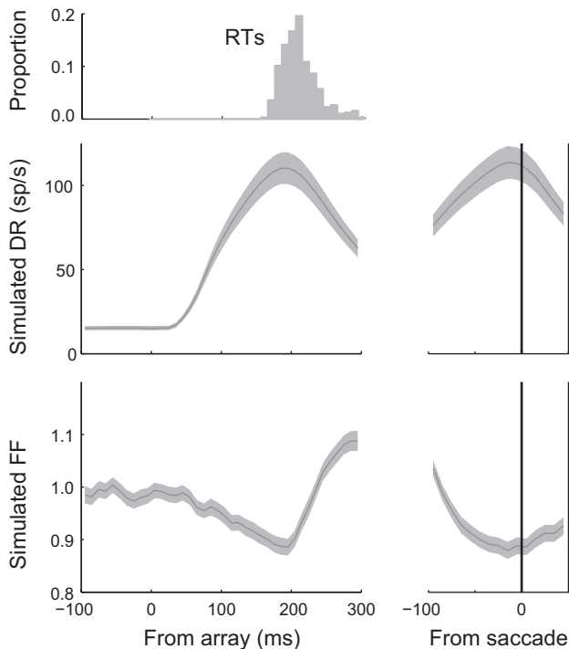
Fig. 11. Accumulator model simulations. Simulated model discharge rates ( middle ) and Fano factor ( bottom ) relative to array onset ( left ) and saccade ( right ). Lines are the averages ( \pm SE) across 304 simulated neurons with 110 simulated trials to match the statistical power of the observed data. Gray histogram ( top ) is the quantile averaged response time (RT) probability distribution across all simulations. Only 1 accumulator representing a saccade to the neurons' RF was simulated. Note that Fano factor begins declining \sim 50 ms after target onset and reaches a minimum at the time of saccade initiation as observed in frontal eye field (FEF) neurons (see Fig. 10, C and D ).
