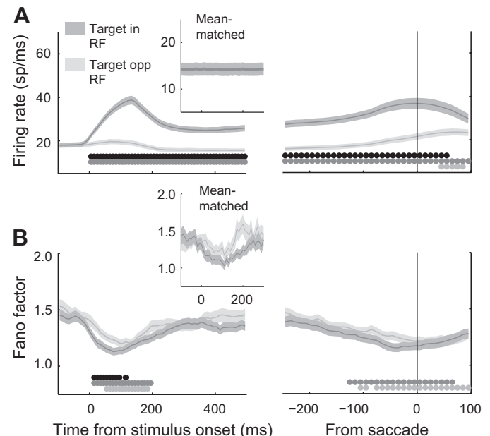
Fig. 12. Memory-guided saccades. Mean discharge rate ( A ) and Fano factor ( B ) during memory-guided saccades aligned to target onset ( left ) or saccade ( right ) in which the target appeared inside (dark gray; Target in RF) or diametrically opposite (light gray; Target opp RF) the neurons' RFs. Stimulus duration was 80–150 ms, and delay intervals ranged from 500 to 1,000 ms. Insets show mean-matched discharge rate and Fano factor. Conventions are as described in Fig. 2.
