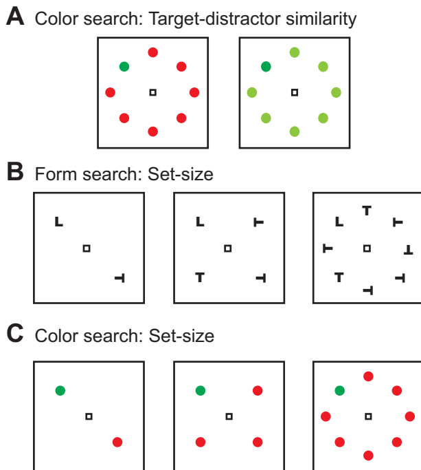
Fig. 1. Color and form visual search tasks. After fixation for a variable delay, a search array appeared consisting of a target and distractors. Monkeys were trained to make a single saccade to the location of the target for reward. A: color search task with target-distractor similarity manipulation. Monkey F searched for a green or red target. Target-distractor similarity varied across trials. Target color varied across sessions. B: form search task with set size manipulation. Monkeys Q and S searched for a rotated L among Ts or T among Ls. Set size varied across trials (2, 4, and 8 stimuli). Target identity was consistent within a session. Stimuli were arranged such that 1 distractor was always diametrically opposite the target location. C: color search task with set size manipulation. Monkeys Q and S searched for a green or red target among red or green distractors, respectively. The task was otherwise identical to the form search task.
