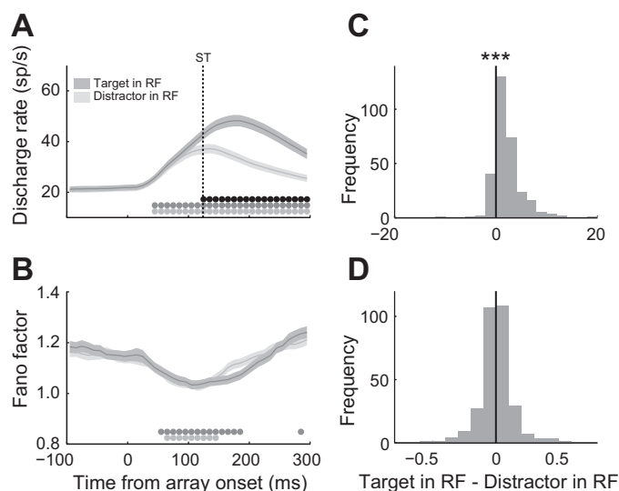
Fig. 2. Temporal dynamics of discharge rate and Fano factor aligned on array onset for the full population of 304 neurons during all visual search tasks. A : mean discharge rate (lines) and \pm SE (shading) was computed in a 50-ms sliding window separately for trials in which the target or a distractor was in the receptive field (RF). Gray circles indicate significance from baseline (100 ms before array onset) in steps of 10 ms when the target (dark gray) or distractors (light gray) were in the RF (Wilcoxon ranked-sum test, P < 0.01 ). Black circles indicate significant differences between discharge rates when the target or distractors were in the RF. Dotted vertical line indicates the selection time (ST), which is the time when the distribution of discharge rates for trials in which the target vs. distractor were in the RF first diverged significantly for 5 consecutive time bins. B : mean Fano factor computed in same analysis windows as described above. There is no ST labeled because the distribution of Fano factors for trials in which the target vs. distractor were in the RF never significantly diverged. The brief but nonsignificant separation around \sim 190 ms can be attributed to saccade initiation. C : distribution of differences in discharge rate when the target or a distractor was in the neurons' RFs computed in the poststimulus epoch 100 ms after array presentation until 100 ms before mean saccade response time. *** P < 0.001 , significant difference from 0 (Wilcoxon signed-rank test). D : distribution of differences for Fano factor.
