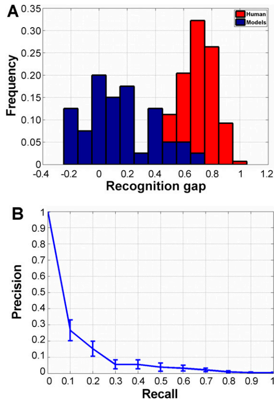
Fig. 57. Models' recognition gap and performance. (A) Distributions of the recognition gap (between MIRCs and their similar but unrecognized sub-MIRCs) by humans and by computational models (average gap over all MIRC and sub-MIRC pairs of the same class). (B) Models performance: Precision recall curve of the computational models' training of full-object images (average of four classifiers). The error bars show the SD for each recall rate.
