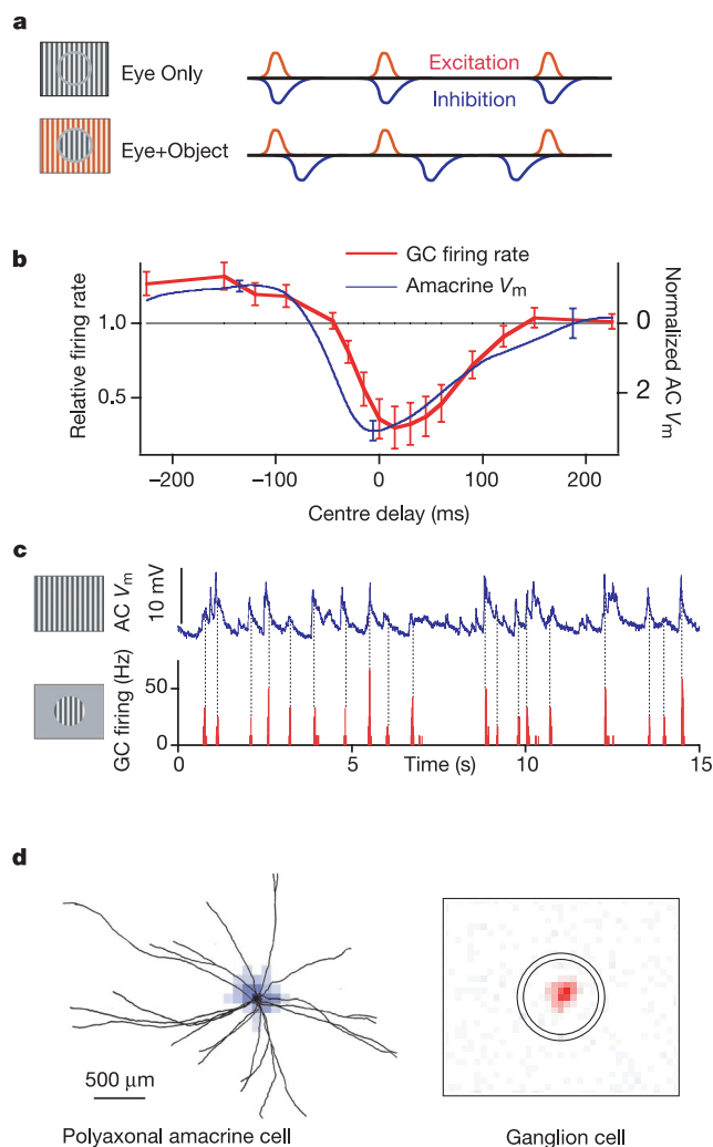
Figure 4 Transient excitation and inhibition are synchronous during coherent motion, causing suppression of firing. a , Schematic proposal for the inputs to an OMS ganglion cell: excitation from motion in the receptive field centre, and inhibition from motion in the periphery. Both consist of transient events and are triggered by the same motion features. Under coherent motion they coincide in time, but under incoherent motion they are uncorrelated. b , Average firing rate of Fast OFF ganglion cells (GCs) as the jitter trajectories of the object and background regions are shifted in time relative to each other (thick red line). Firing rates were averaged over 5-min stimulus presentations, normalized to the cell’s average firing rate under the Object Only condition, then averaged over five neurons. Average membrane potential of polyaxonal amacrine cells ( AC V_m ) during global (Eye Only) jitter, as a function of time before or after a ganglion cell spike in the Object Only condition using the same trajectory (thin blue line). Each amacrine cell’s membrane potential was normalized by subtracting its mean and dividing by its standard deviation, which was 4 \pm 1 mV (mean \pm s.e.m.; n = 3 ); note inverted axis, depolarization is downward. c , Membrane potential of a polyaxonal amacrine cell in response to coherent motion (top; Eye Only condition). Spiking response of a salamander Fast OFF cell to motion in the Object Only condition, using the same trajectory as for the amacrine cell (bottom). The amacrine and ganglion cells were recorded in different retinas. d , Vertical projection of the confocal image of the amacrine cell in c , superimposed on its receptive field (left). Receptive field of the ganglion cell in c , on the same scale (right).
