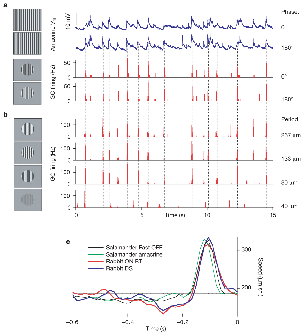
Figure 5 The response of OMS cells is largely independent of the spatial pattern. a , Responses of a salamander polyaxonal amacrine cell (top) and a Fast OFF ganglion cell (bottom) to a jittering grating ( 0^\circ ) and its contrast-reversed version ( 180^\circ ). b , Responses of a different Fast OFF ganglion cell to a grating of varying spatial period. c , The average time course of the retinal speed of the jittered grating before a spike for a salamander
