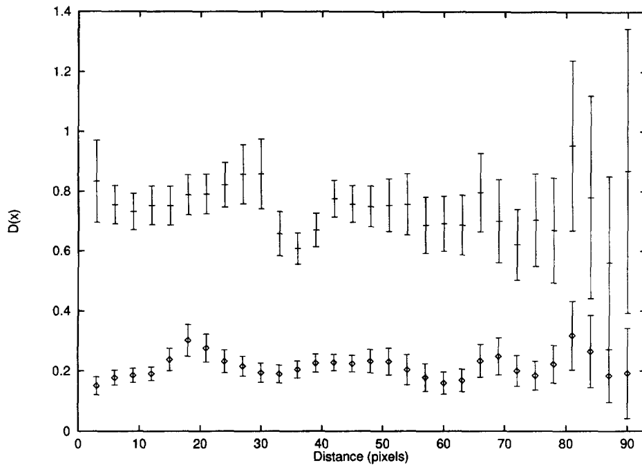
FIGURE 4. The difference functions D_{\text{diff}}(x) (upper) and D_{\text{same}}(x) (lower). Neither obeys a significant linear trend, and so they can be approximated by constants.
