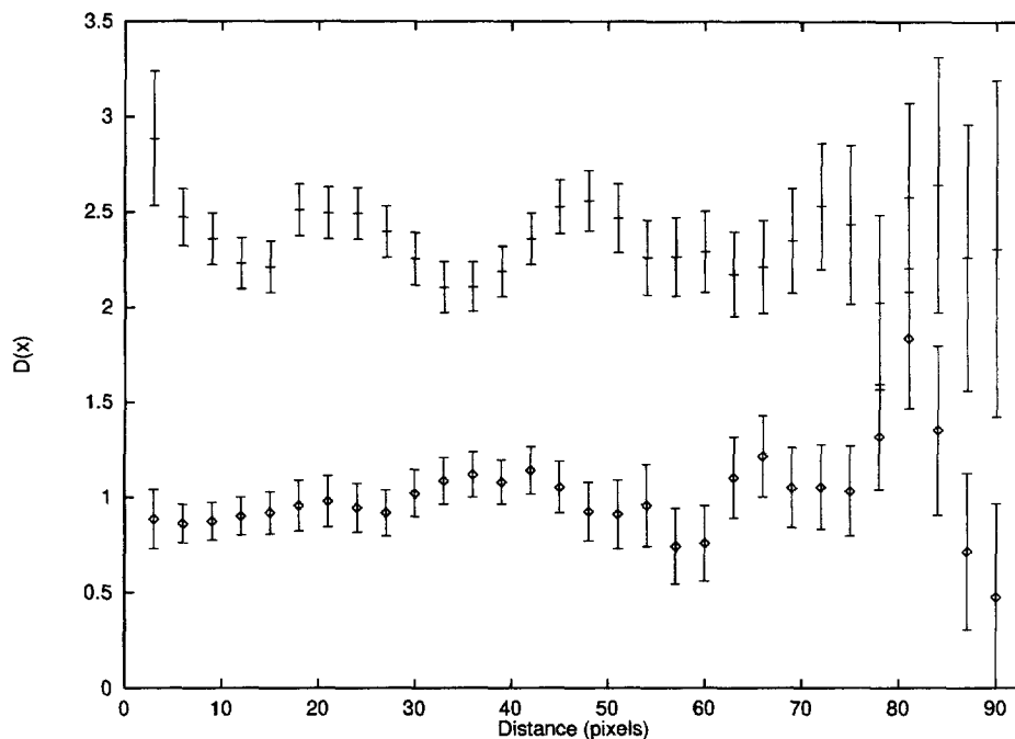
FIGURE 6. The difference functions D_{\text{diff}}(x) (upper) and D_{\text{same}}(x) (lower) for the same image locations as Fig. 4, but with the images recalibrated to black-and-white pixel values. The difference functions remain essentially flat to within error bars.
