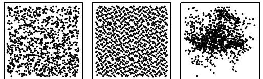
Figure 3: The first 1000 points of: a uniformly random sample (left), the Sobol sequence (center), and a Brownian random walk with standard deviation 0.1 (right).
