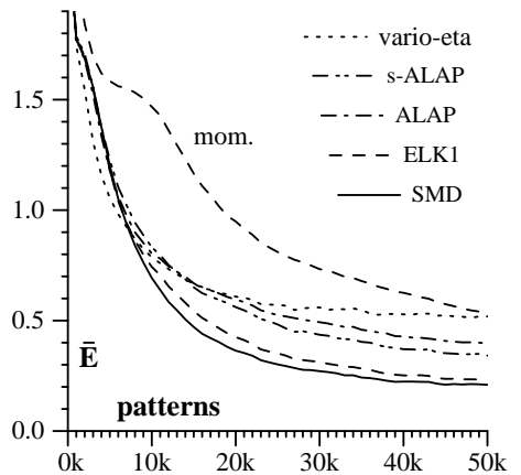
Figure 2: The average smoothed loss \bar{E} during online training on the four regions task, plotted against the number of training patterns (uniformly random sampling).
