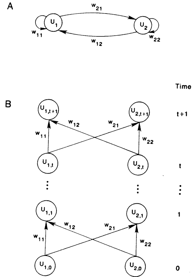
FIGURE 17. A comparison of a recurrent network and a feedforward network with identical behavior. A : A completely connected recurrent network with two units. B : A feedforward network which behaves the same as the recurrent network. In this case, we have a separate unit for each time step and we require that the weights connecting each layer of units to the next be the same for all layers. Moreover, they must be the same as the analogous weights in the recurrent case.
