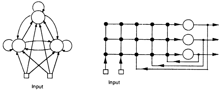
Figure 1. Two representations of a completely connected recurrent network having three units and two input lines. One input line might serve as a bias and carry the constant value 1. Any subset of these three units may serve as output units for the net, with the remaining units treated as hidden units. The 3 \times 5 weight matrix for this network corresponds to the array of heavy dots in the version on the right.
