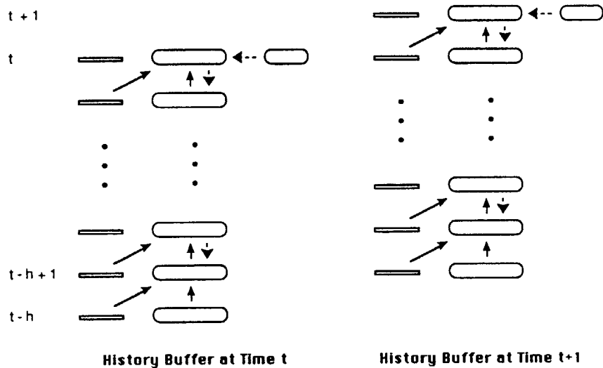
Figure 9. A schematic representation of the storage and processing required for the BPTT(h) algorithm for two consecutive executions of the error gradient computation, one at time step t and the next at time step t + 1 . The history buffer always contains the current network input, activity, and target values, along with the values of network input and activity for the h prior time steps. The BPTT computation requires injection of error only for the current time step and is performed anew at each subsequent time step.
