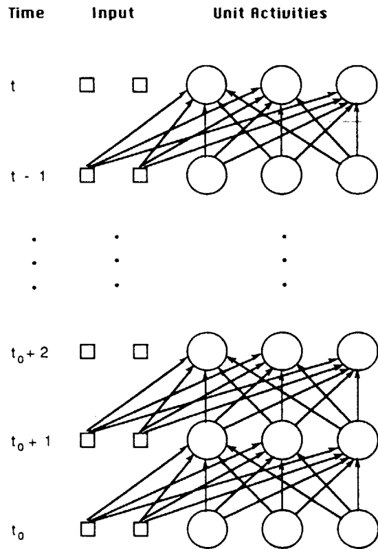
Figure 2. The unrolled version of the network shown in Figure 1 as it operates from time t_0 through time t . Each connection in the network is assumed to have a delay of one time step.
