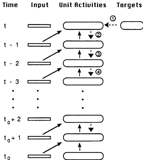
Figure 3. A schematic representation of the storage and processing required for real-time BPTT at each time step t . The history buffer, which grows by one layer at each time step, contains at time t all input and unit output values for every time step from t_0 through t . The solid arrows indicate how each set of unit output values is determined from the input and unit outputs on the previous time step. A backward pass, indicated by the dashed arrows, is performed to determine separate \delta values for each unit and for each time step back to t_0 + 1 . The first step is the injection of external error based on the target values for time step t , and all remaining steps determine virtual error for earlier time steps. Once the backward pass is complete the partial derivative of the negative error with respect to each weight can then be computed.
