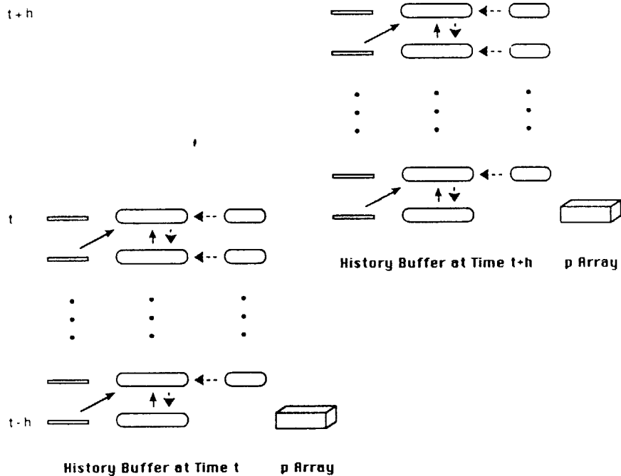
Figure 6. A schematic representation of the storage and processing required for the FP/BPTT( h ) algorithm for two consecutive executions of the error gradient computation, one at time step t and the next at time step t + h . From time step t - h through time step t the network input, activity, and target values are accumulated in the history buffer. At time t the cumulative error gradient is computed on the basis of one BPTT pass through this buffer, also using the p values stored for time step t - h . In addition, n separate BPTT passes, one for each unit in the network, are performed to compute the p values for time t . Each such BPTT pass begins with the injection of 1 as "error" at a single unit at the top level. Once the weights have been adjusted on the basis of the cumulative error gradient over the interval (t - h, t] and the p values have been updated at time t , accumulation of the history begins anew over the interval [t, t + h] .
