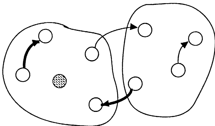
Figure 11. A network divided into two subnetworks for subgrouped RTRL. The full RTRL algorithm requires keeping track of the sensitivity of each unit in the network with respect to each weight in the network. When subgrouping is used, each unit only pays attention to its sensitivity to weights on connections terminating in the group to which it belongs. Thus, among the four connections shown, only those two indicated with the heavy lines are considered when computing the sensitivity of the unit indicated by the shading to variations in the weights.
