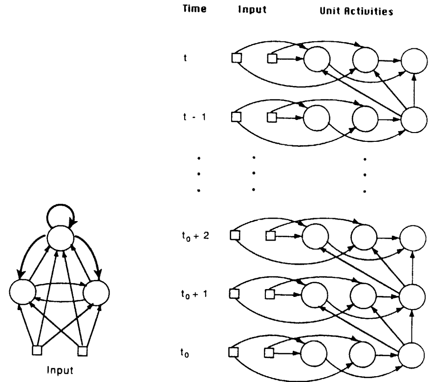
Figure 7. A network having connections with delays of 0 and 1 and its unrolling from time t_0 to t . The feedforward connections, indicated by the thinner arrows in the network itself, all have a delay of 0. These correspond to the within-level connections in the unrolled version. The feedback connections, indicated by the thicker arrows in the network, all have a delay of 1. These correspond to the connections from each level to the next level above it in the unrolled version. Other delays beside 0 and 1 are possible and would be represented by connections that skip levels. In the unrolled network, updating of activity is assumed to occur from left to right within each level and then upward to the next level. Thus a sequence of operations is performed within each single time step when computing the activity in the network. When errors are back-propagated, processing goes in the reverse direction, from higher levels to lower levels and from right to left within each level.
