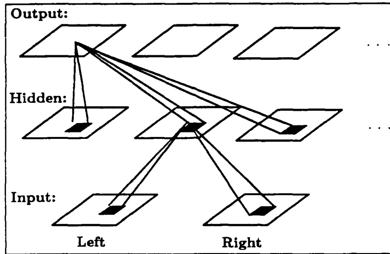
Figure 11.1: Structure of the stereo network. See text for a description.
