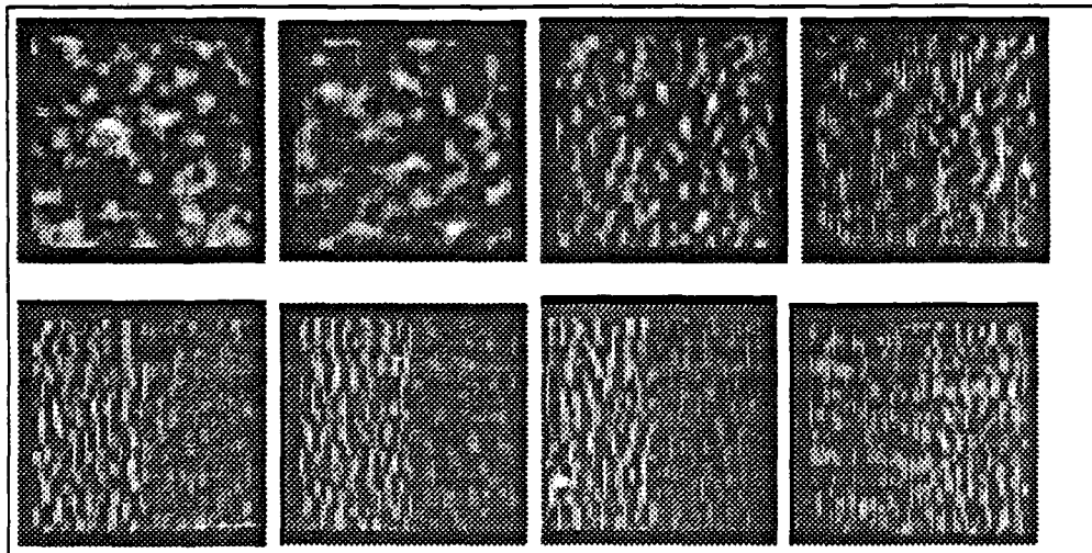
Figure 11.2: Hidden layer response for a two-layer nonlinear network trained on stereo images. The left half of the input random dot image has a 2 pixel disparity, and the right half has zero disparity.
