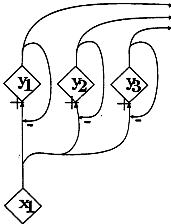
Figure 3.2: Network implementation of the Generalized Hebbian Algorithm.
