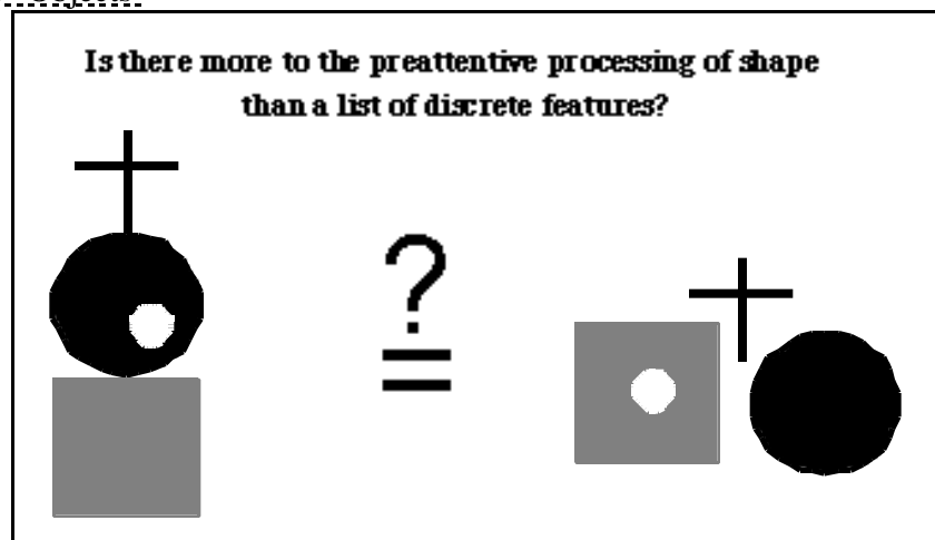
Figure Thirteen - A problem in the preattentive analysis of form.
