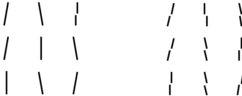
Figure 10: It is easy to find an vernier offset even among stimuli with different orientations (10a). It is much harder to find the stimulus with the vernier offset to the right among distractors with offsets to the left (10b).
