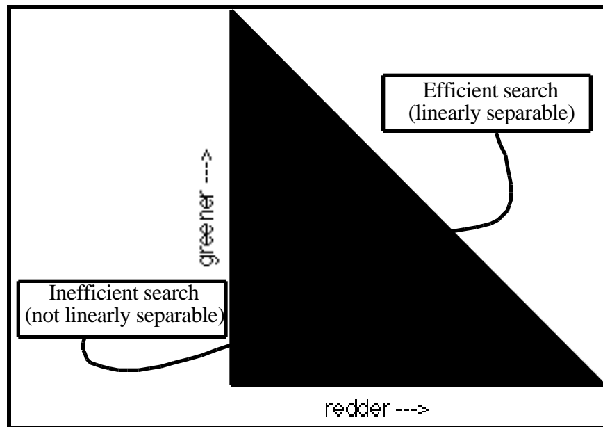
Figure Seven: Linear separability in color space.
