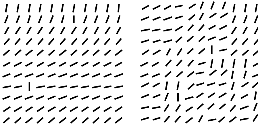
Figure Eight: Find the two vertical lines in each array.
