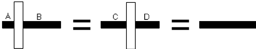
Figure Fourteen: Preattentive processes know about occlusion.
