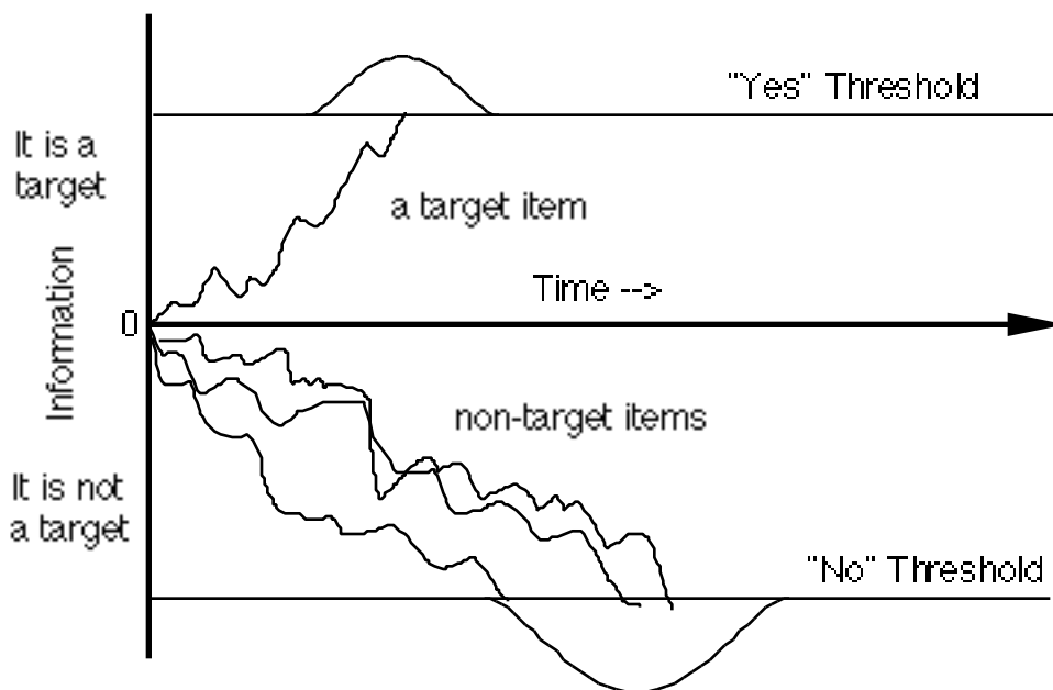
Figure Four - A Limited-Capacity Parallel Model
