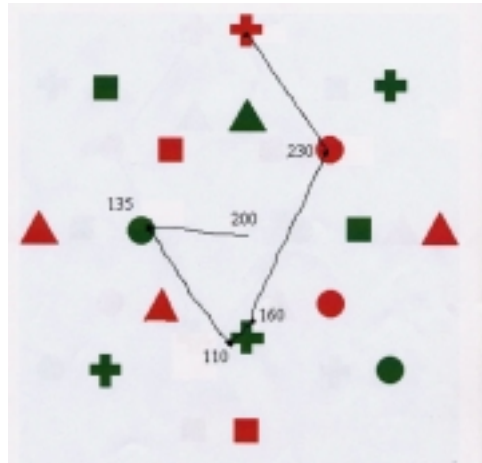
FIGURE 5.5. Feature-conjunction search task of the type studied by Findlay (1997), together with a record of a subject's eye-scan data. The target in this display was a cross located in the centre-top of the display, and subjects were instructed to move their eyes to the target as rapidly as possible. The figures show the fixation times in milliseconds for fixations before the target was reached.
