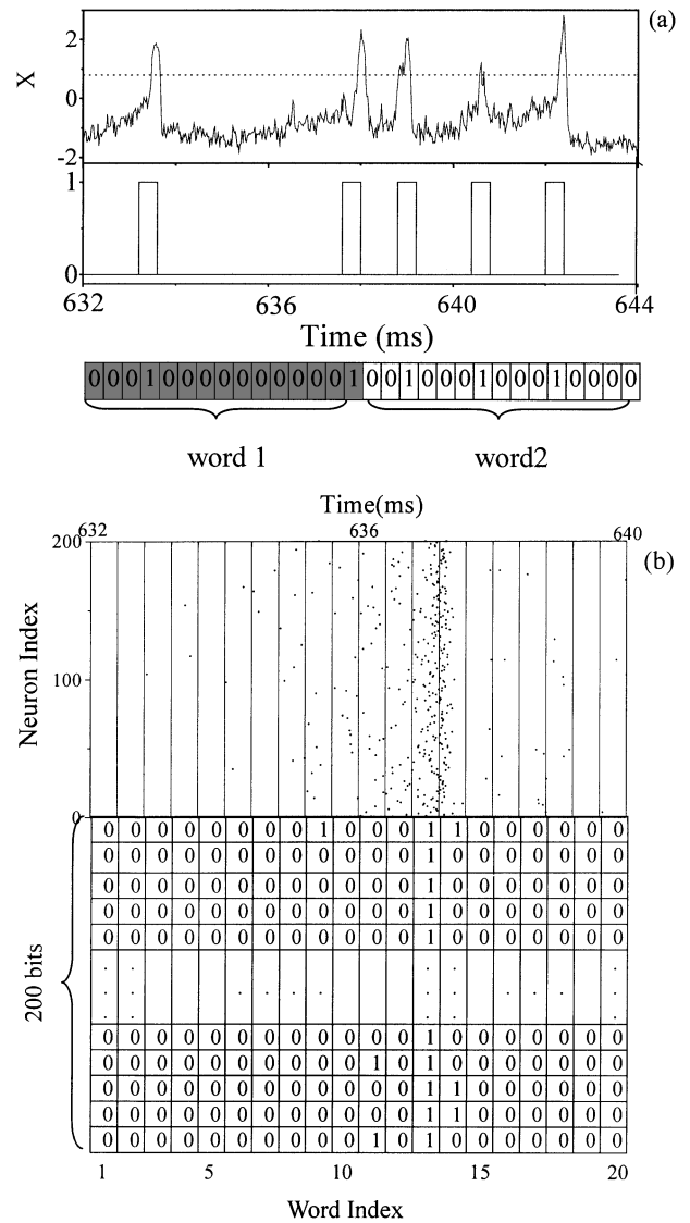
Fig. 1. Schematic of the calculation of the entropy correlated (a) with the spike train of a neuron and (b) with the temporal firing patterns of neurons.
