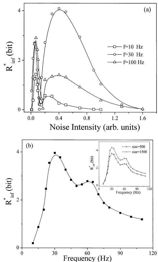
Fig. 3. (a) R_{inf}^* vs the noise intensity for the signals with f_s = 10 ( \square ), 30 ( \circ ), and 100 Hz ( \nabla ), respectively. (b) R_{inf}^* vs the signal frequency in the case of D = 0.5 with 750 and 500 as well as 1500 (in the inset) words analyzed, respectively.
