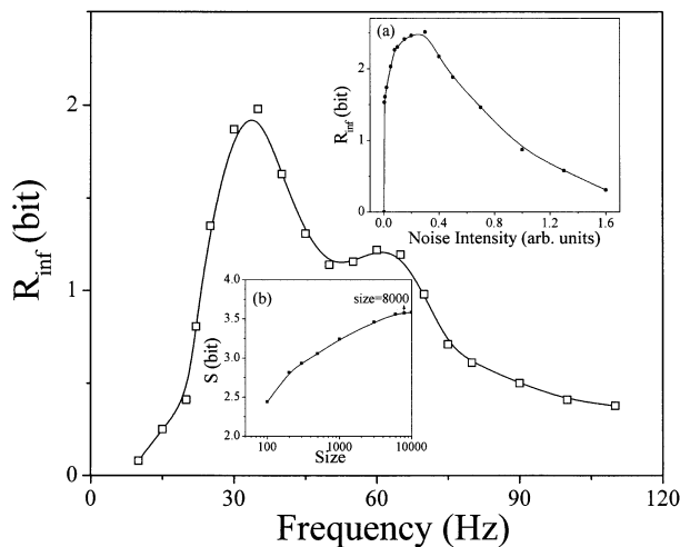
Fig. 2. R_{inf} vs the signal frequency in the case of D = 0.5 for the 1st element within the network. The inset (a) is R_{inf} vs the noise intensity in the case of f_s = 30 Hz and (b) is the entropy S vs the data size in the case of f_s = 30 Hz and D = 0.5 .
