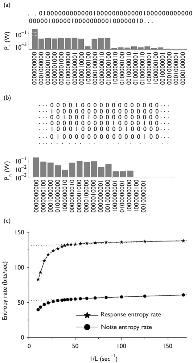
Fig. 3. Illustration of calculation of mutual information rate. (a) Probability distribution of words P_r(W) of length L=10 with time bin \delta t=2 ms, for the calculation of H_r . P(W) for W=0000000000 is far off scale (0.84). Although 2^{10} patterns were possible, only 23 words actually occurred ( n=50000 ). Inset, samples of one sequence composed of different words. (b) Probability distribution of words P_n(W) of length L=10 with time bin \delta t=2 ms, at one time position in 500 repeated trials of one neuron, for the calculation of H_{noise} . Over 500 repeats, only 16 different words were observed. Inset, samples from 6 of the 500 trials to the repeated stimulus. A particular 10-bin word at time t is highlighted. (c) Estimated total response entropy rate H_r and noise entropy rate H_{noise} are plotted as a function of the reciprocal of word length, 1/L . Both H_r and H_{noise} decrease gradually with increase of L implying of correlations between bins. The drop of the two curves for large L indicates the distortion effect due to the limited data. Dashed dotted lines show the extrapolations from the linear part of these curves to infinitely long words [22]. Mutual information is obtained by the difference between the two extrapolation values [22].
