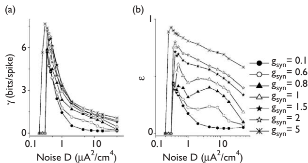
Fig. 5. (a) Information transmission rate \gamma as a function of noise intensity D for various coupling strengths. (b) Coding efficiency \epsilon as a function of noise intensity D for various coupling strengths.
