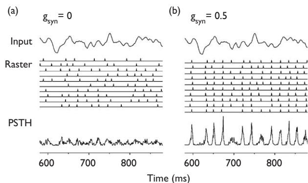
Fig. 2. (a) In the presence of noise D=5 , the network with g_{syn}=0 for input aperiodic stimulus s(t) (upper) displays noisy firing activities (see middle raster plot for 10 neurons). The peaks in the PSTH of total 1000 neurons (lower plot) are weak and random. (b) In the presence of noise D=5 , the network with g_{syn}=0.5 for input aperiodic stimulus s(t) (upper) displays ordered firing activities (see middle raster plot for 10 neurons). The peaks in the PSTH of total 1000 neurons (lower plot) are high and phase locked.
