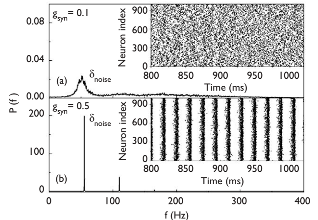
Fig. 1. PSDs of V^*(t) and the raster plots of firings of the neurons for D = 5 , and g_{syn} = 0.1 (a), 0.5 (b), respectively.
