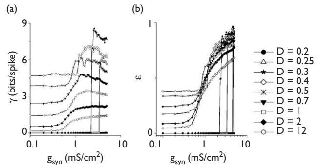
Fig. 4. (a) Information transmission rate \gamma as a function of coupling strength g_{syn} for various noise intensities. (b) Coding efficiency \epsilon as a function of coupling strength g_{syn} for various noise intensities.
