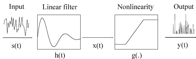
Fig. 1. The LN model consists of a linear filter h(t) followed by a nonlinearity g(\cdot) . x(t) is the convolution of the input signal s(t) and the filter h(t) . The nonlinearity g(\cdot) operates on x(t) to generate the output y(t) .
