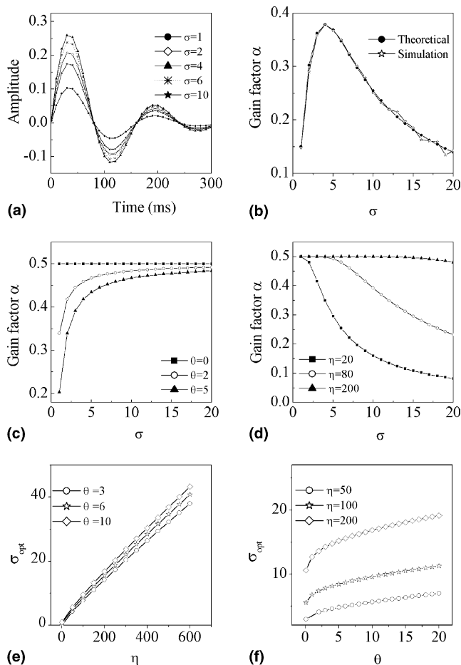
Fig. 2. (a) The theoretical kernels recovered from stimuli of different \sigma for threshold \theta = 3 and saturation \eta = 50 . (b) The gain factor \alpha as a function of \sigma . (c) The gain factor \alpha as a function of \sigma for three threshold values with \eta = 1000 . (d) The gain factor \alpha as a function of \sigma for three saturation values with \theta = 0 . (e) The \sigma where \alpha reaches maximum is called \sigma_{opt} . \sigma_{opt} increases linearly with saturation level \eta for different threshold values ( \theta = 3, 6 and 10 ). (f) For fixed saturation levels ( \eta = 50, 100 and 200 ), \sigma_{opt} increases monotonically, but not linearly, with threshold \theta .
