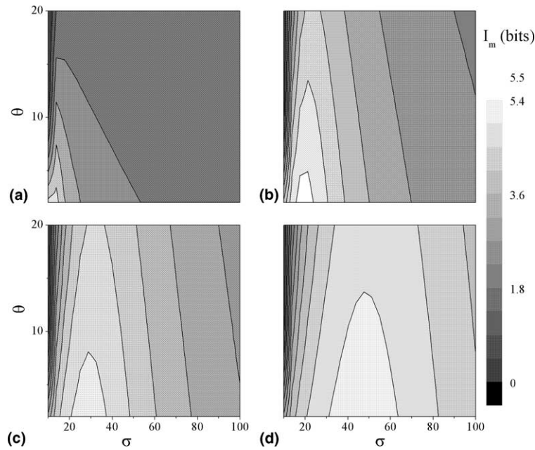
Fig. 6. Mutual information I_m(\sigma, \theta) for \eta = 20 (a), \eta = 100 (b), \eta = 200 (c), and \eta = 400 (d) respectively.
