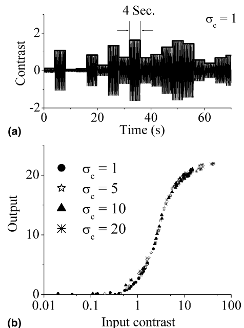
Fig. 5. For the model with \theta = 5 and \eta = 50 : (a) A example of input contrast signal with sinewave modulation (temporal sine frequency is 10 Hz). The standard deviation of contrasts is \sigma_c = 1 . (b) Input–output relations for various input contrast signals with \sigma_c = 1, 5, 10 and 20 , respectively.
