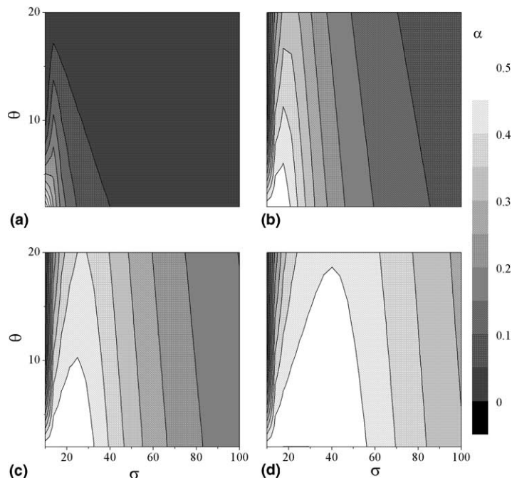
Fig. 3. Gain factor \alpha(\sigma, \theta) for \eta = 20 (a), \eta = 100 (b), \eta = 200 (c), and \eta = 400 (d) respectively.
