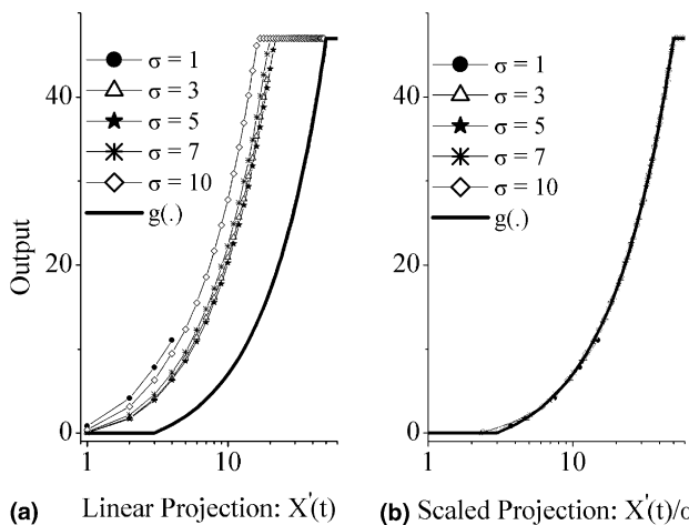
Fig. 4. (a) The recovered nonlinearities for various values of \sigma in the case of \theta = 3 and \eta = 50 . (b) Scaled nonlinearities by gain factor \alpha for various values of \sigma in the case of \theta = 3 and \eta = 50 .
