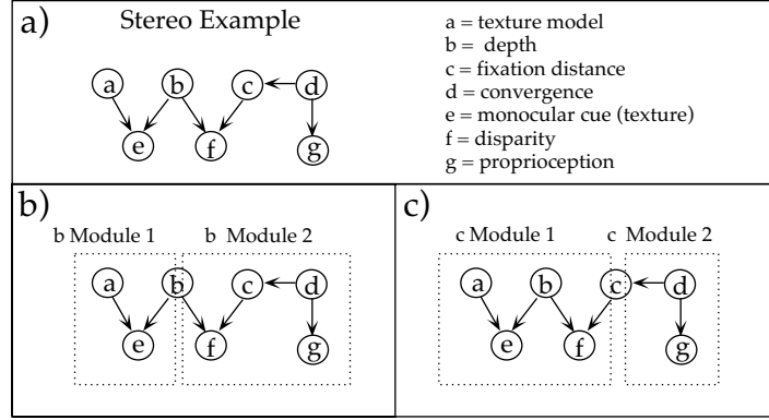
Figure 5: Example Bayes Net. a) Bayes net representing the factored distribution p(a, b, c, d, e, f, g) = p(a)p(b)p(c|d)p(d)p(e|a,b)p(f|b,c)p(g|d) . The graphical model can express the probabilistic structure of depth from stereo and texture inference. b) When estimating the depth variable b , the Net can be decomposed into two separate depth modules (depth from texture and depth from stereo). The dashed boxes show the modules. c) When estimating the fixation distance c , the net can be decomposed into two separate distance modules (distance from texture and stereo, and distance from proprioception). Note that the left hand side of the graph does not decompose as before. This illustrates Bayesian modularity (see Section 4.3).
